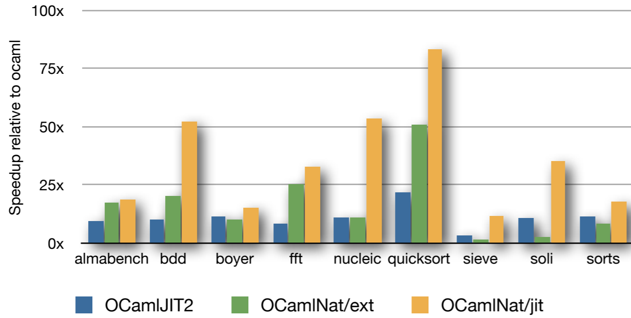
MacBook Pro Core i7, OS X 10.7 (amd64)
