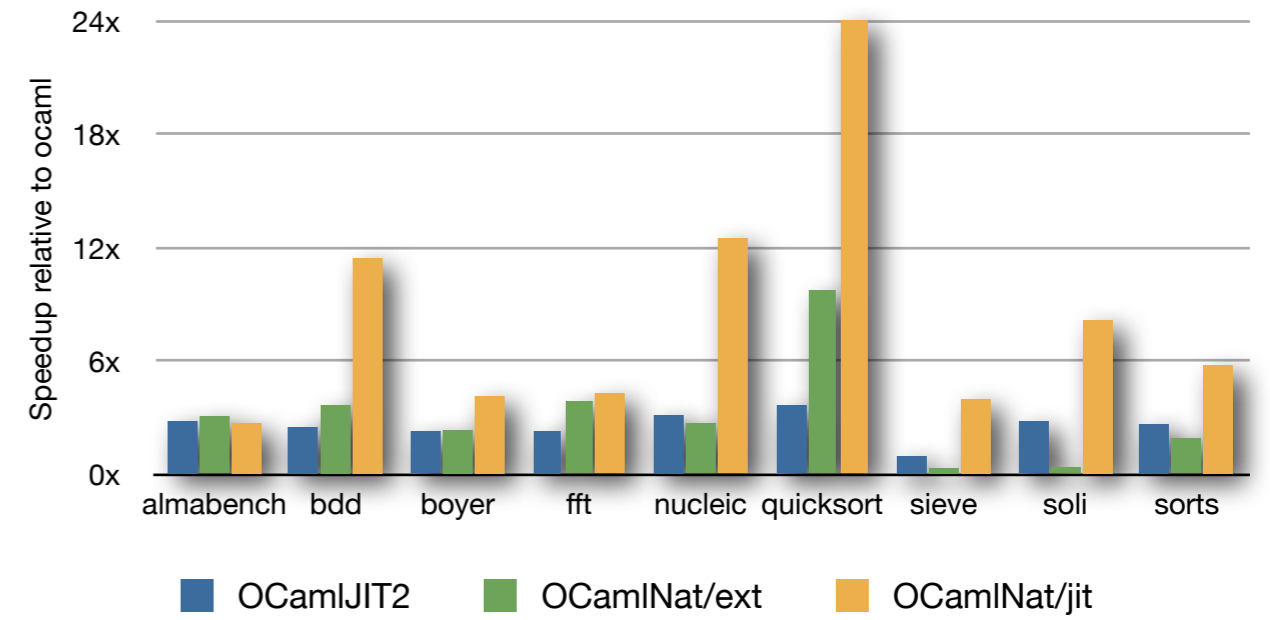
Pentium 4, Debian testing 2011/09/14 (i386)
