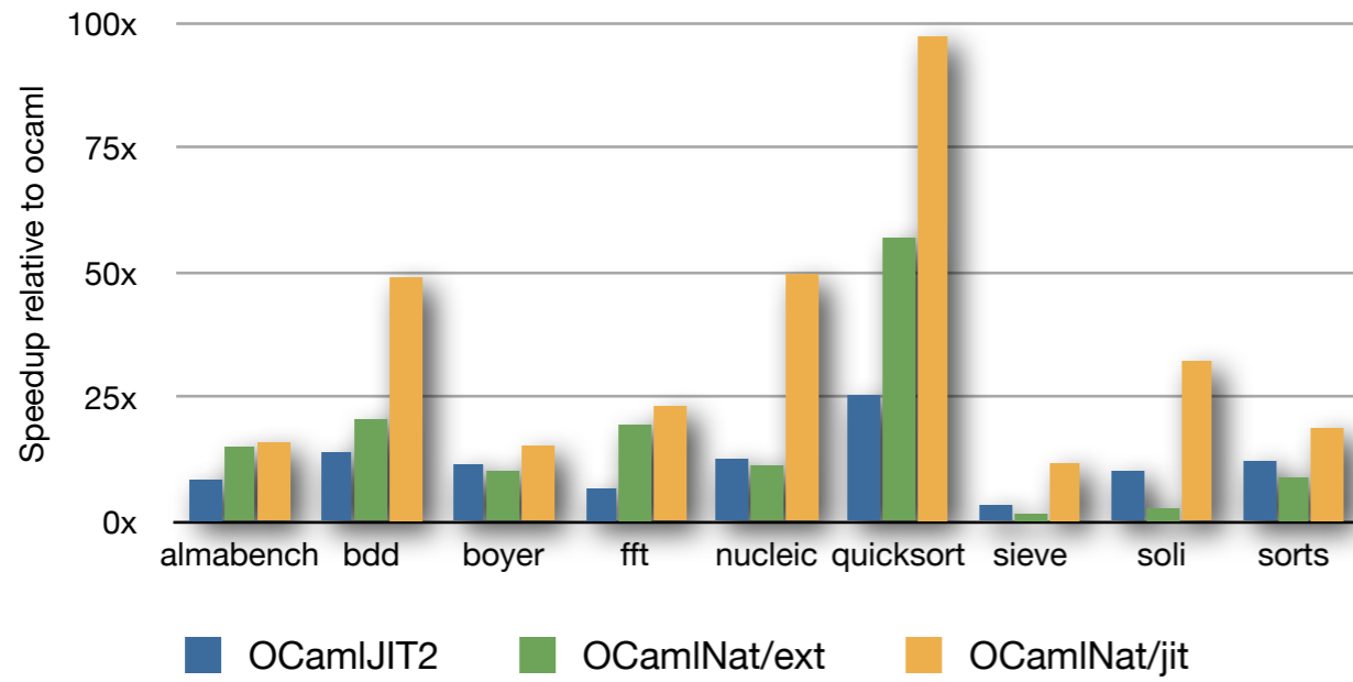
MacBook Core 2 Duo, OS X 10.7 (amd64)
