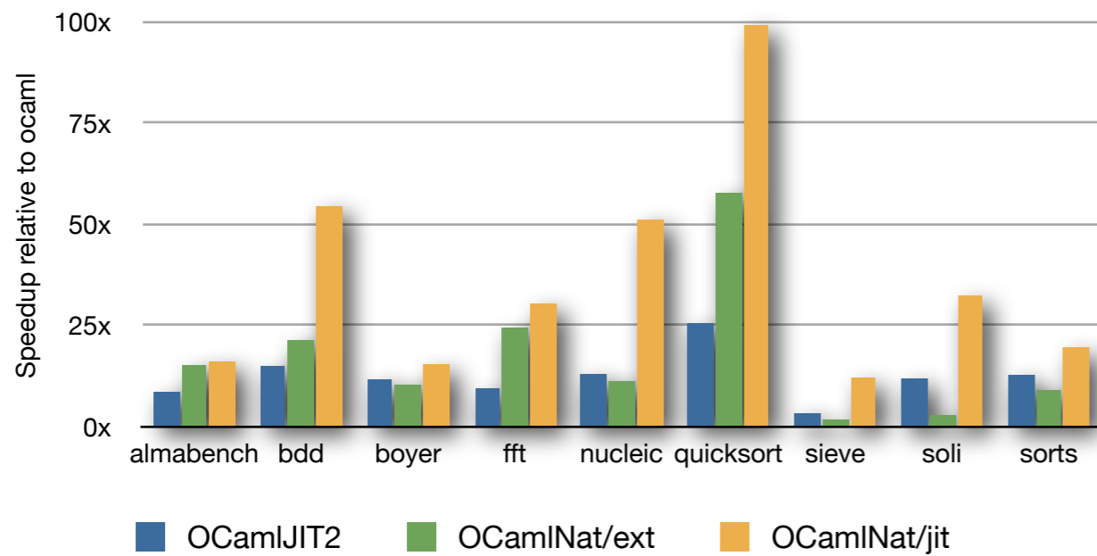
iMac Core 2 Duo, OS X 10.7 (amd64)
